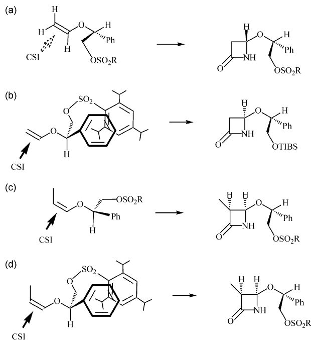
Figure 3. Preferred stereochemical pathway for cycloaddition of CSI to vinyl ethers and Z -propenyl ethers. For the sake of simplicity, configuration of substrates refer to ( R ) series only. 18
