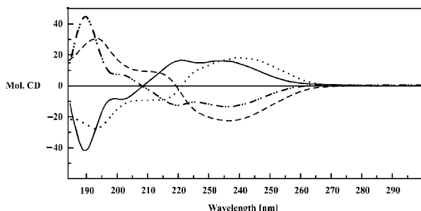
Figure 2. CD spectra of clavams 32 (—), 33 (---), 50 (.....), and 51 (— · — · —) recorded in acetonitrile.
