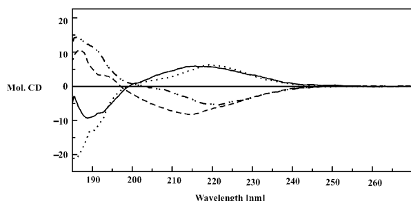
Figure 1. CD spectra of azetidinones 24 (.....), 25 (---), 46 (— · — · —), and 47 (—) recorded in acetonitrile.
